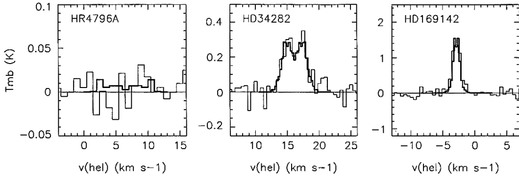
FIG. 1. CO J = 3-2 spectra for HR 4796A, HD 34282, and HD 169142, overlaid with model spectra (thin and thick histograms, respectively). For HR 4796A the model is for the maximum-allowed gas mass, constrained by the CO upper limit and the orbital velocities in a 50–125 AU radius disk. The models for the two stars are for the minimum gas masses, as described in the text.
